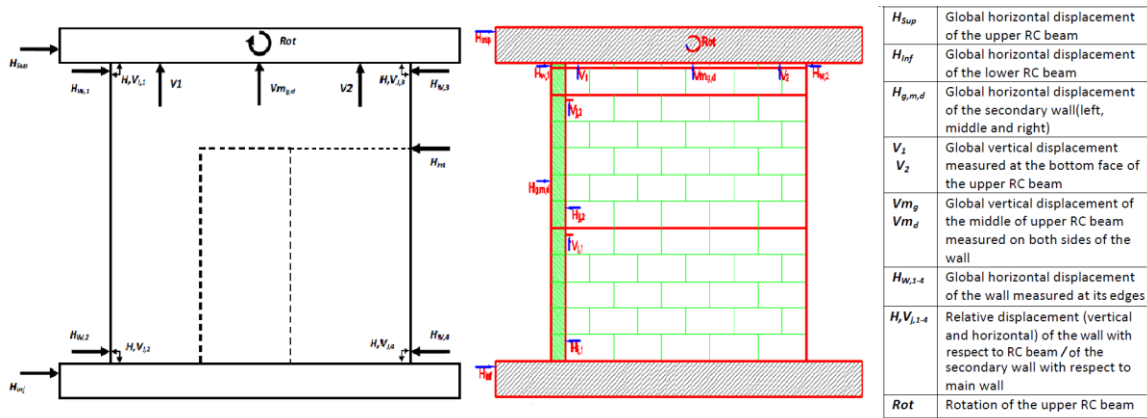
Figure 4. Instrumentation layouts of the specimens
