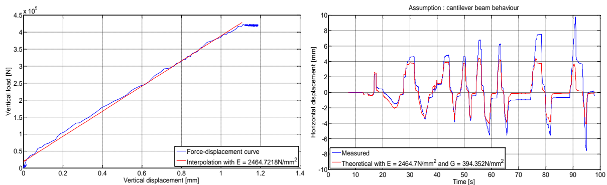
Figure 8. Assessment of the elastic (left) and shear (right) moduli
