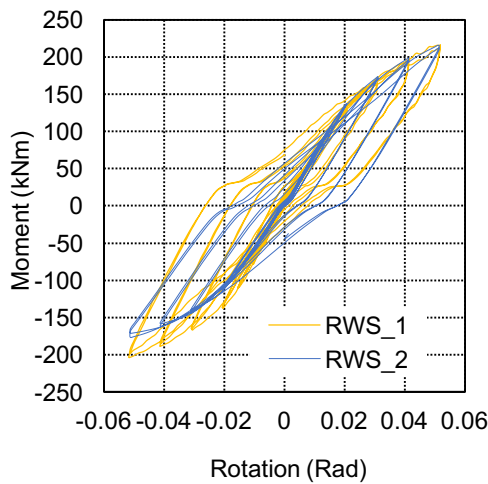
Figure 4. Hysteretic graph of RWS_1/RWS_2 Figure 5. Hysteretic graph of RWS_3/RWS_4
