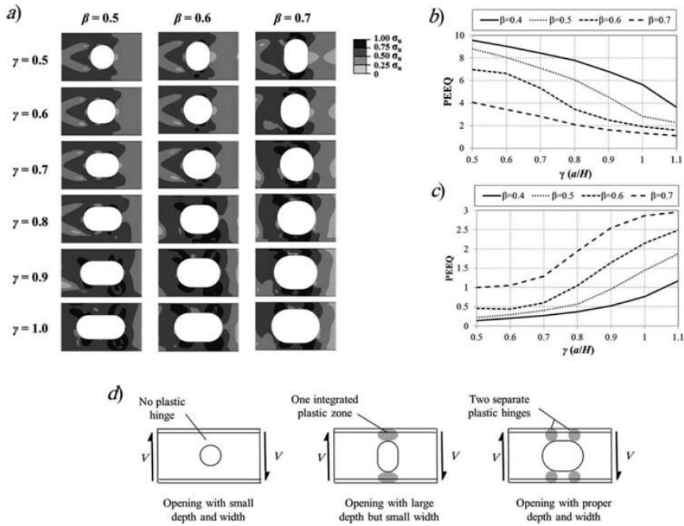
Figure 1. Effect of opening depth and length on: (a.) stress-strain distribution (b.) Equivalent plastic strain at connection welds (c.) equivalent plastic strain at opening corners (d.) Critical failure modes (Erfani and Akrami, 2016)
