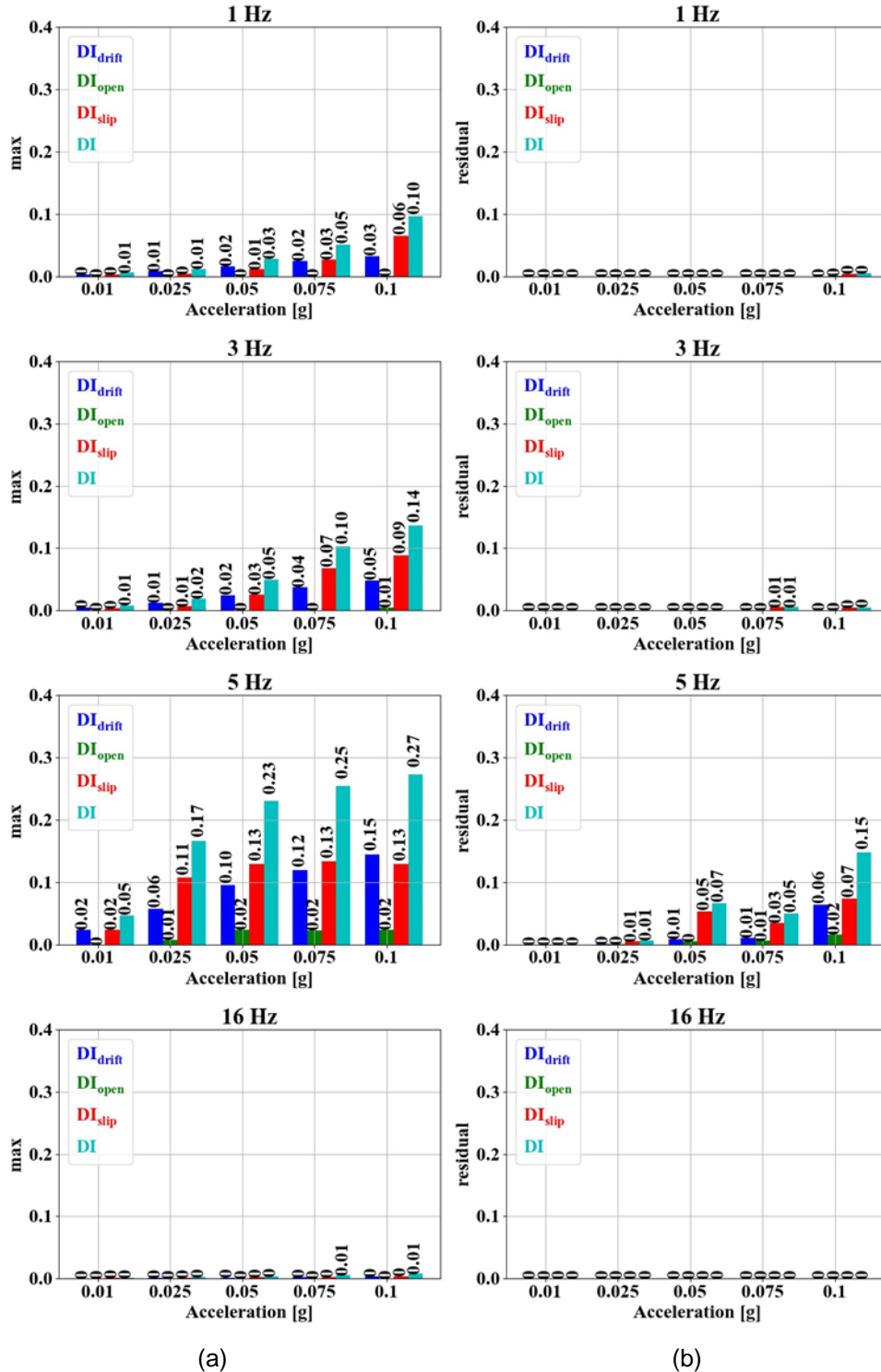
Figure 3: Maximum (a) and residual (b) DI_{drift} , DI_{open} , DI_{slip} and DI presented for the case of the wall with the symmetric opening. Each graph corresponds to a different value of frequency (1, 3, 5 and 16Hz).
