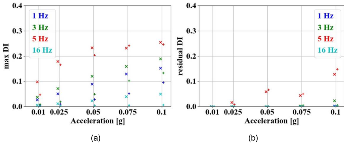
Figure 2: Numerical results of the maximum (a) and residual (b) DI in the masonry walls with respect to the applied amplitude of acceleration and frequency. The results for the symmetric and asymmetric models are shown as '+' and 'x' accordingly.
